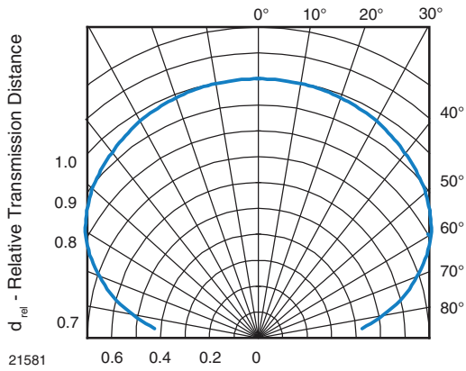
Fig. 11 - Horizontal Directivity
