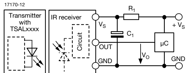
R_1 and C_1 recommended to reduce supply ripple for V_S < 2.2 V
