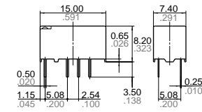
Self clinching terminal
