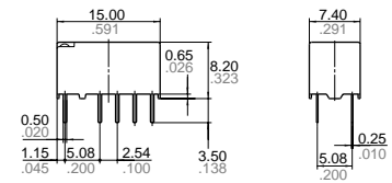
Self clinching terminal
