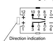
2 coil latching (L2)
