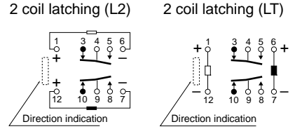
Schematic (Bottom view)
