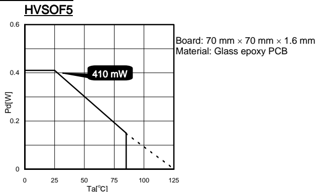
Fig. 26 HVSO5 Power Dissipation/Power Dissipation Reduction (Example)
