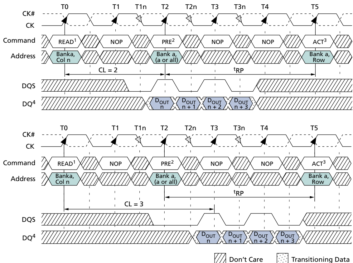
Figure 37: READ-to-PRECHARGE
