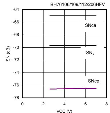
Fig.25 Supply Voltage-S/N
