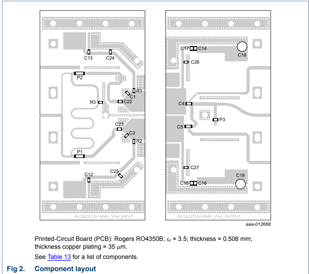
Fig 2. Component layout
