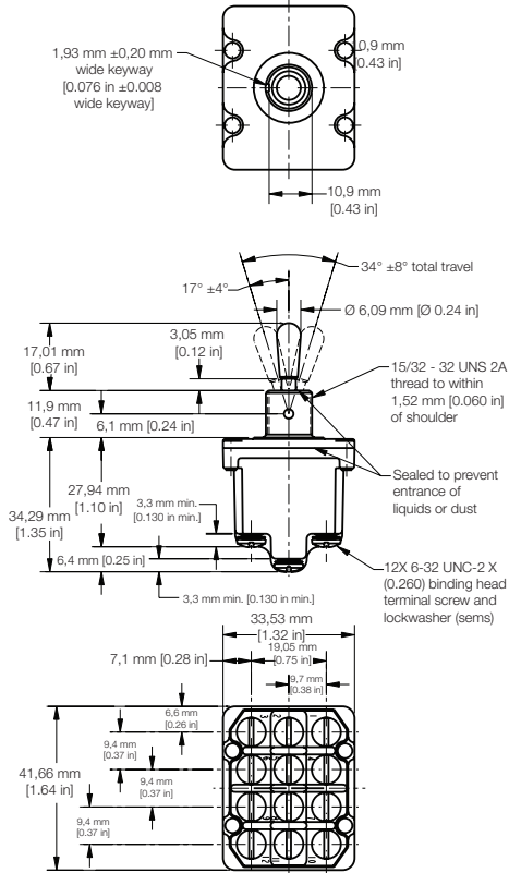
4TL1: Four-pole, standard lever, screw terminals
