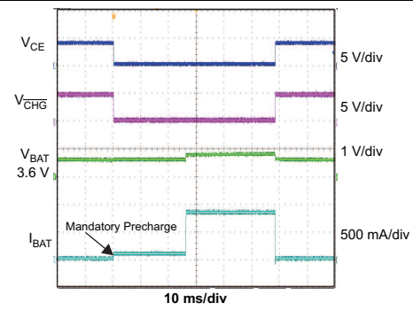
Figure 29. Charger On/Off Using \overline{CE}
