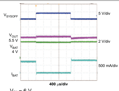
Figure 31. BQ24075T, BQ24079T System On/Off With Input Connected
