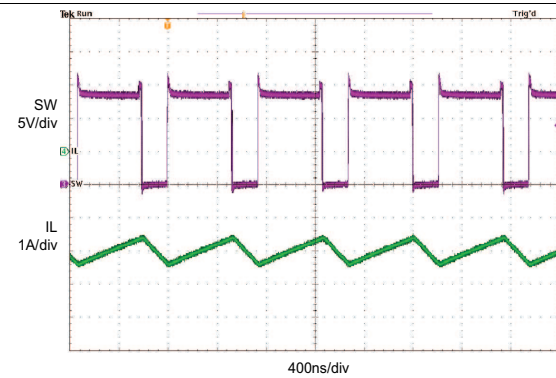
Figure 44. PWM Switching Waveform
