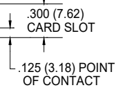
SINGLE ROW CONTACTS READ ONE SIDE OF DAUGHTER BOARD
