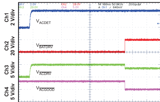
t - Time = 100 ms/div Figure 18.
