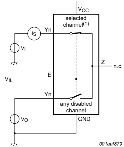
(1) Channel is selected by S0, S1 and S2. Fig. 5. Test circuit for measuring ON-state leakage current
