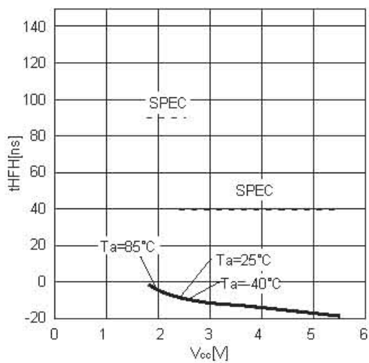
Figure 26. HOLD setting hold time t_{HFH}
