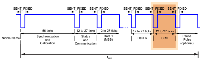
Figure 42: CRC Nibble within the SENT Message Frame
