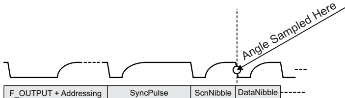
Figure 52: Sample-on-Output Example
