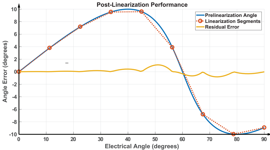
Figure 8: Post-Linearization Error
