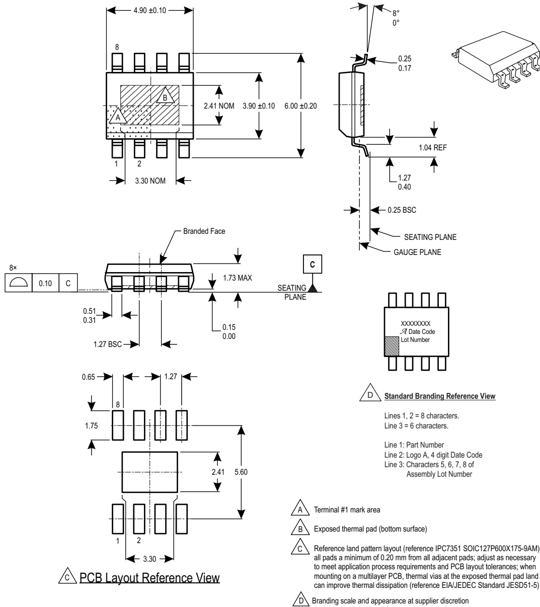
Figure 5: Package LJ, 8-Pin eSOIC
