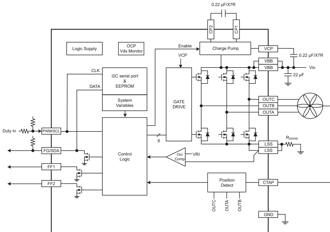
Figure 1: Typical Application
