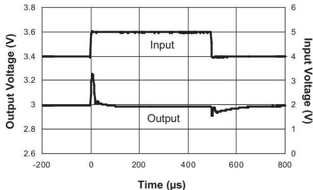
Line Response With 100mA Load
