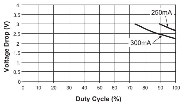
Device Duty Cycle vs. V_{DROP} ( V_{OUT} = 3.0\text{V} @ 50^\circ\text{C} )
