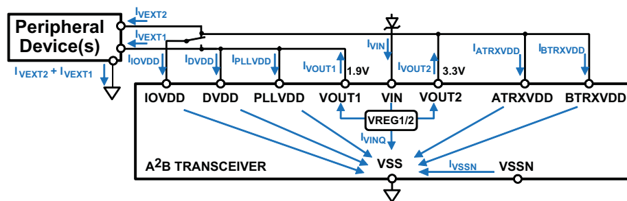
Figure 34. Current Flow Model
