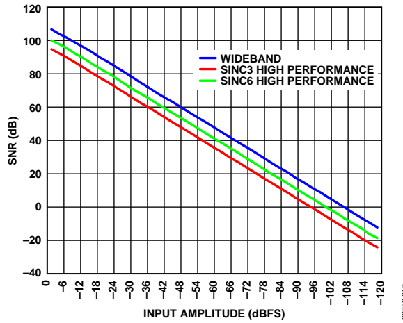
Figure 18. SNR vs. Input Amplitude, Tone at 1 kHz
