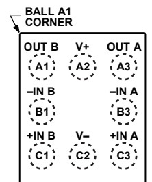
Figure 2. 6-Ball WLCSP (CB-6-7)
