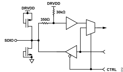
Figure 40. Equivalent SDIO Input Circuit
