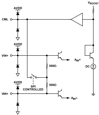
Figure 34. Analog Input DC Equivalent Circuit ( V_{CML} \sim 1.7\text{ V} )
