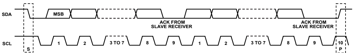
Figure 61. Acknowledge Bit
