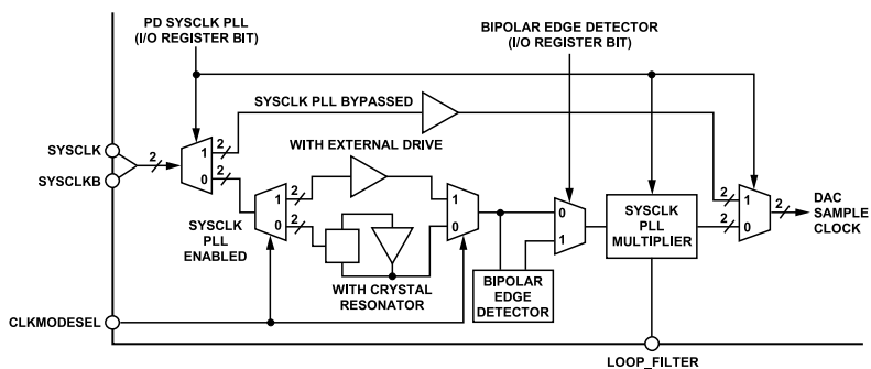
Figure 44. System Clock Generator Block Diagram
