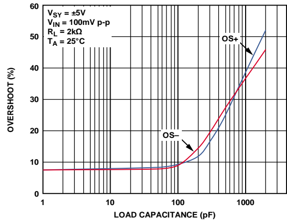
Figure 63. Overshoot vs. Load Capacitance
