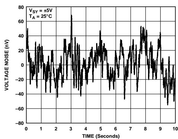
Figure 64. Voltage Noise, 0.1 Hz to 10 Hz
