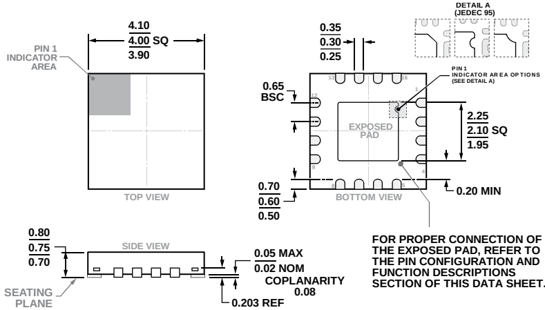
Figure 69. 16-Lead Lead Frame Chip Scale Package [LFCSP] 4 mm × 4 mm Body and 0.75 mm Package Height (CP-16-23) Dimensions shown in millimeters
