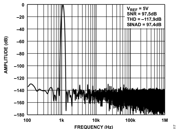
Figure 15. 1 kHz, -0.5 dBFS Input Tone FFT, Wide View, Differential, G = 0.909, V_{REF} = 5V , Low Power Mode
