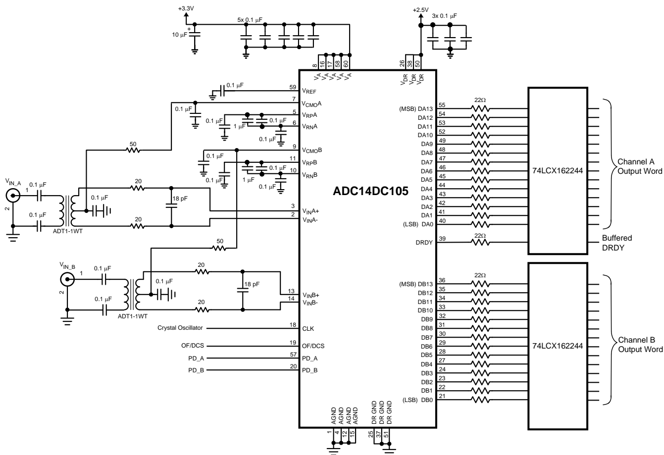
Figure 22. Application Circuit
