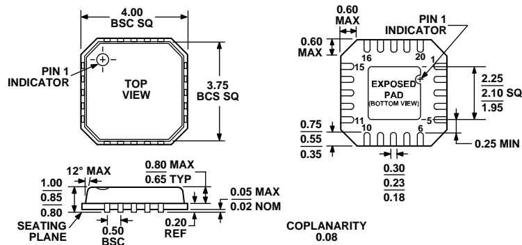
Figure 32. 20-Lead Lead Frame Chip Scale Package [LFCSF_VQ]
