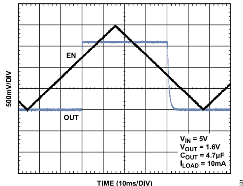
Figure 31. ADP1706 Typical EN Pin Operation
