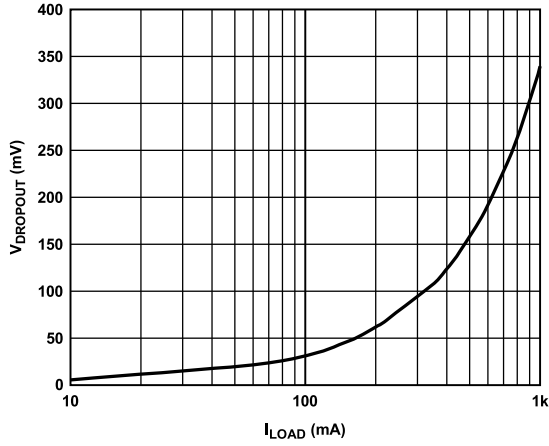
Figure 16. Dropout Voltage ( V_{DROP} ) vs. Load Current ( I_{LOAD} )
