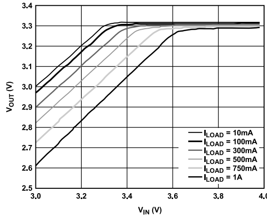
Figure 17. Output Voltage ( V_{OUT} ) vs. Input Voltage ( V_{IN} ) (in Dropout)
