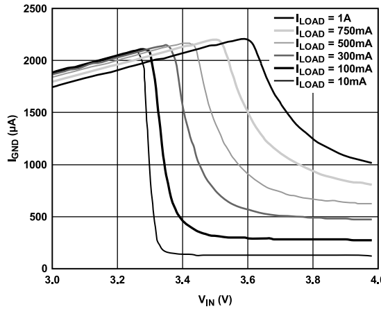
Figure 18. Ground Current ( I_{GND} ) vs. Input Voltage ( V_{IN} ) (in Dropout)
