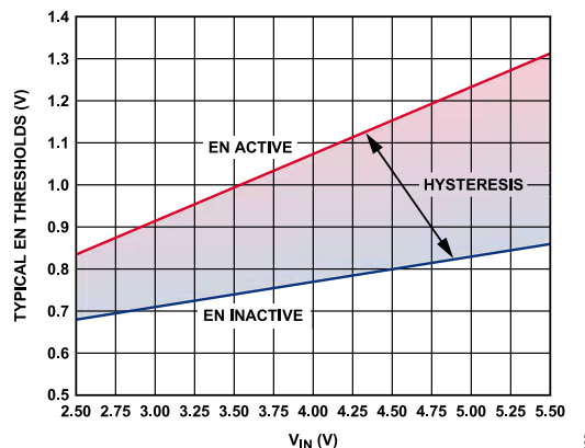
Figure 32. Typical EN Pin Thresholds vs. Input Voltage
