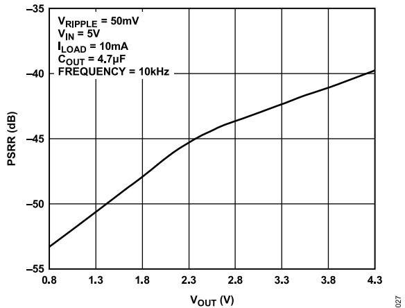
Figure 26. ADP1708 Power Supply Rejection Ratio (PSRR) vs. Output Voltage ( V_{OUT} )
