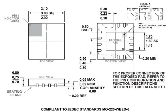
Figure 47. 16-Lead Lead Frame Chip Scale Package [LFCSP] 3 mm x 3 mm Body and 0.75 mm Package Height (CP-16-22) Dimensions shown in millimeters
