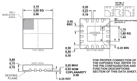
COMPLIANT TO JEDEC STANDARDS MO-220-WEED-6 Figure 47. 16-Lead Lead Frame Chip Scale Package [LFCSP] 3 mm x 3 mm Body and 0.75 mm Package Height (CP-16-22) Dimensions shown in millimeters
