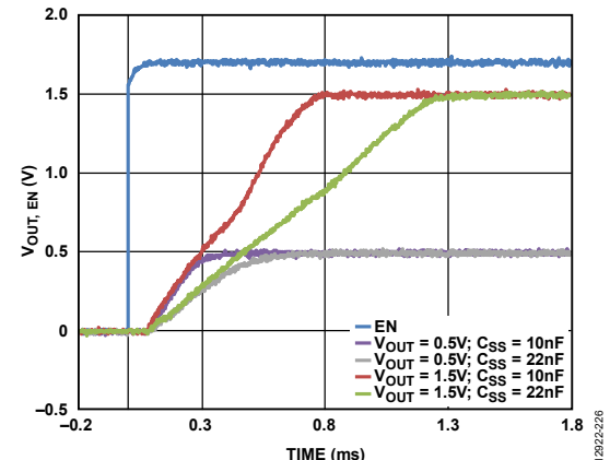
Figure 26. Adjustable V_{OUT} Ramp-Up with External Soft Start Capacitor ( V_{OUT,EN} ) vs. Time
