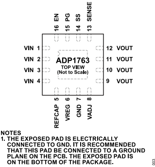
Figure 3. Pin Configuration
