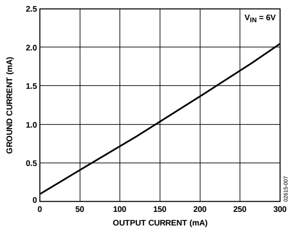
Figure 7. Ground Current vs. Output Current
