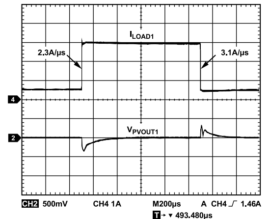
Figure 32. Buck Load Transient, V_{PVIN1} = 12\text{ V} , V_{PVOUT1} = 1.2\text{ V} , I_{LOAD1} = 0.5\text{ A} to 3\text{ A} , f_{SW} = 0.6\text{ MHz} , L = 2.2\text{ μH} , R_C = 3.48\text{ kΩ} , C_C = 2\text{ nF} , C_{CP} = 22\text{ pF} , C_{PVOUT1} = 44\text{ μF}
