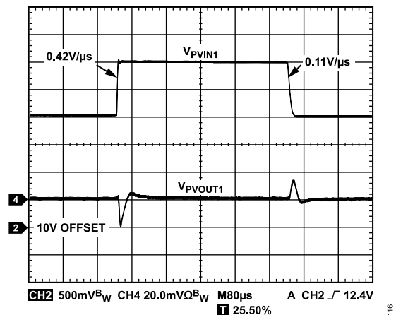
Figure 29. Buck Line Transient, V_{PVIN1} = 12\text{ V} to 13\text{ V} , V_{PVOUT1} = 1.2\text{ V} , I_{LOAD1} = 1\text{ A} , f_{SW} = 0.6\text{ MHz} , L = 2.2\text{ μH} , R_C = 3.48\text{ kΩ} , C_C = 2\text{ nF} , C_{CP} = 22\text{ pF} , C_{PVOUT1} = 44\text{ μF}
