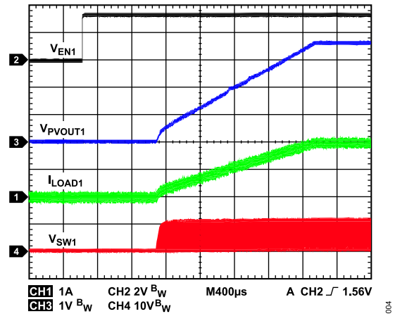
Figure 28. Buck Startup, V_{PVOUT1} = 3.3\text{ V} , I_{LOAD1} = 3\text{ A} ( V_{EN1} is the EN1 Voltage)
