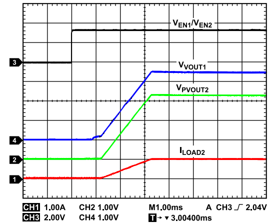
Figure 31. Adaptive Mode Startup, V_{PVOUT2} = 3.3\text{ V} , I_{LOAD2} = 1\text{ A} ( V_{EN2} is the EN2 Voltage)
