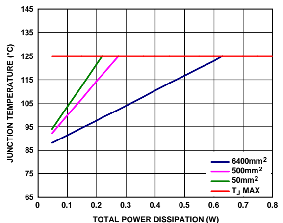
Figure 57. SOIC, T A = 85°C
