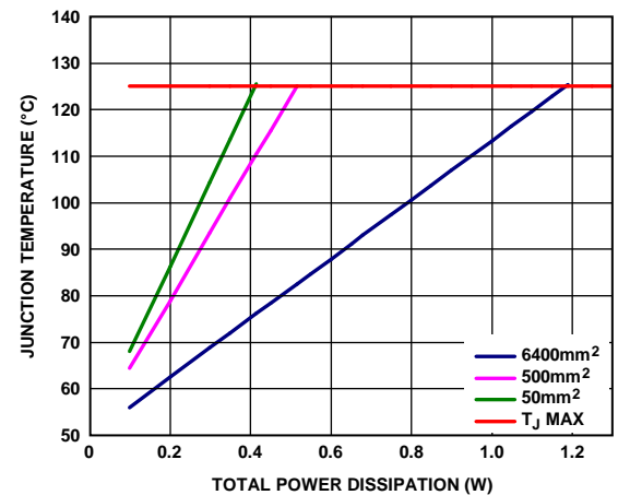
Figure 56. SOIC, T A = 50°C
