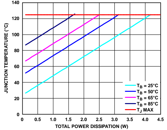
Figure 55. SOIC, T A = 25°C
