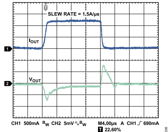
Figure 33. Load Transient Response, I_{LOAD} = 100\text{ mA} to 1.2\text{ A} , V_{OUT} = 3.3\text{ V} , V_{IN} = 4.0\text{ V} , C_{OUT} = 22\text{ }\mu\text{F} , Channel 1 = I_{OUT} , Channel 2 = V_{OUT}
