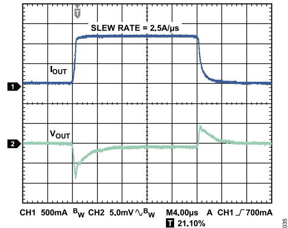
Figure 32. Load Transient Response, I_{LOAD} = 100\text{ mA} to 1.2\text{ A} , V_{OUT} = 3.3\text{ V} , V_{IN} = 4.0\text{ V} , Channel 1 = I_{OUT} , Channel 2 = V_{OUT}
