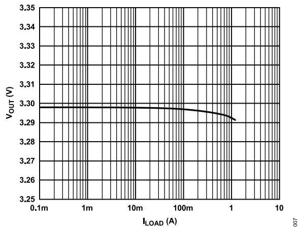
Figure 6. Output Voltage ( V_{OUT} ) vs. Load Current ( I_{LOAD} ), V_{OUT} = 3.3\text{ V}
