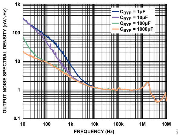
Figure 29. Noise Spectral Density vs. Frequency at Various Values of C_{BYP}
