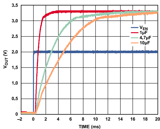
Figure 51. Typical Start-Up Behavior with C_{BYP} = 1\text{ }\mu\text{F} to 10\text{ }\mu\text{F}
