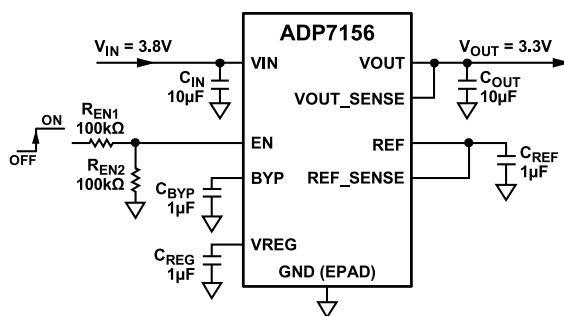
Figure 50. Typical EN Pin Voltage Divider
