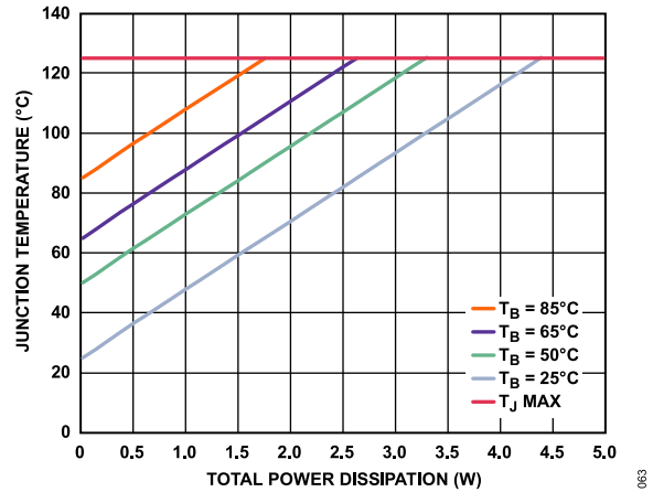
Figure 60. Junction Temperature vs. Total Power Dissipation for the 8-Lead SOIC
