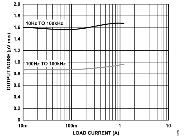
Figure 27. RMS Output Noise vs. Load Current
