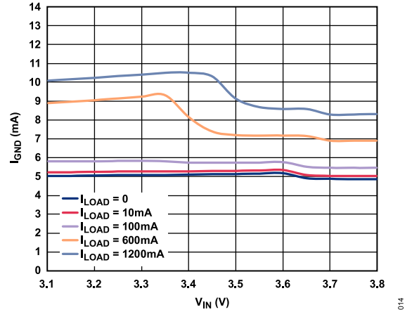
Figure 13. Ground Current ( I_{GND} ) vs. Input Voltage ( V_{IN} ) at Various Loads in Dropout, V_{OUT} = 3.3\text{ V}
