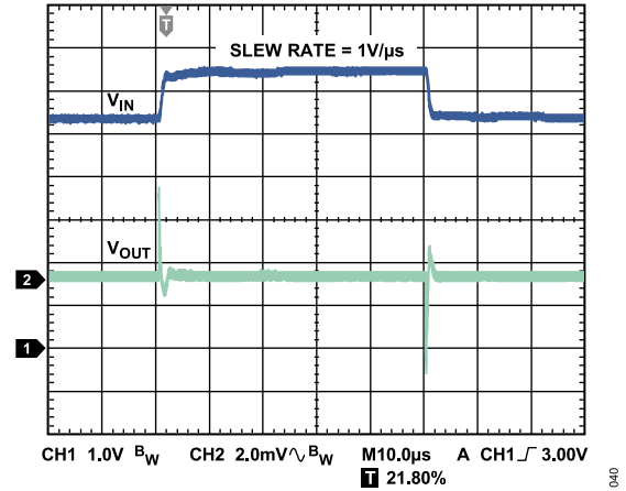
Figure 37. Line Transient Response, 1\text{ V} Input Step, I_{LOAD} = 1.2\text{ A} , V_{OUT} = 1.8\text{ V} , V_{IN} = 2.5\text{ V} , Channel 1 = V_{IN} , Channel 2 = V_{OUT}
