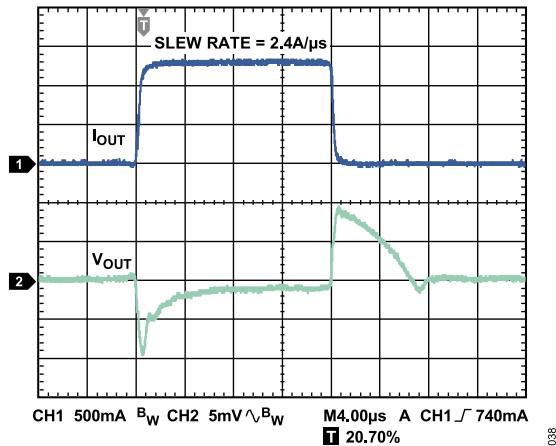
Figure 35. Load Transient Response, I_{LOAD} = 100\text{ mA} to 1.2\text{ A} , V_{OUT} = 1.8\text{ V} , V_{IN} = 2.5\text{ V} , C_{OUT} = 22\text{ }\mu\text{F} , Channel 1 = I_{OUT} , Channel 2 = V_{OUT}
