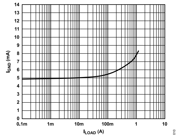
Figure 9. Ground Current ( I_{GND} ) vs. Load Current ( I_{LOAD} ), V_{OUT} = 3.3\text{ V}
