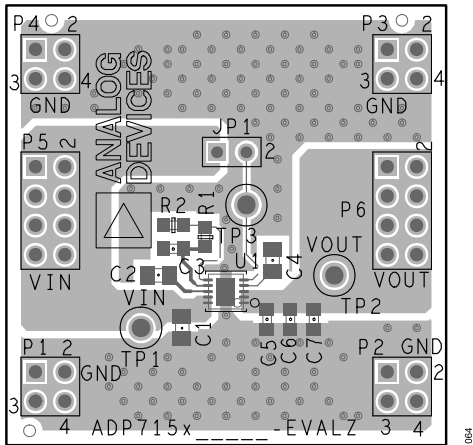
Figure 61. Sample 10-Lead LFCSP PCB Layout
