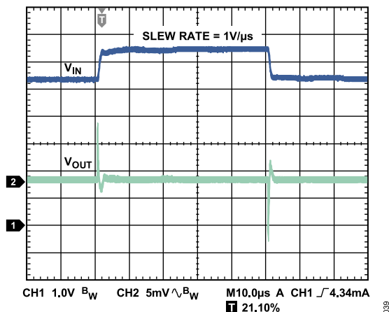
Figure 36. Line Transient Response, 1\text{ V} Input Step, I_{LOAD} = 1.2\text{ A} , V_{OUT} = 3.3\text{ V} , V_{IN} = 3.8\text{ V} , Channel 1 = V_{IN} , Channel 2 = V_{OUT}
