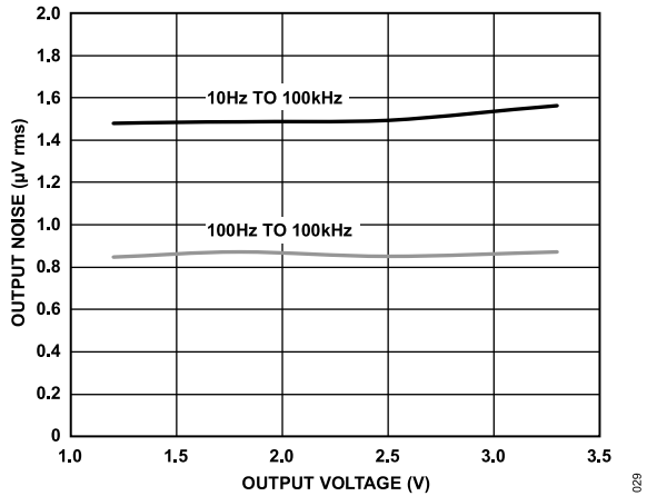
Figure 28. RMS Output Noise vs. Output Voltage
