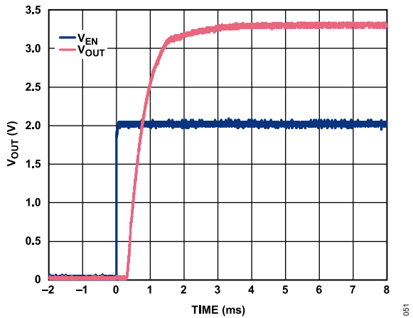
Figure 48. Typical V_{OUT} Response to EN Pin Operation ( V_{EN} , V_{OUT} = 3.3\text{ V} , V_{IN} = 5\text{ V} , C_{BYP} = 1\text{ }\mu\text{F} )
