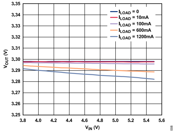
Figure 7. Output Voltage ( V_{OUT} ) vs. Input Voltage ( V_{IN} ) at Various Loads, V_{OUT} = 3.3\text{ V}
