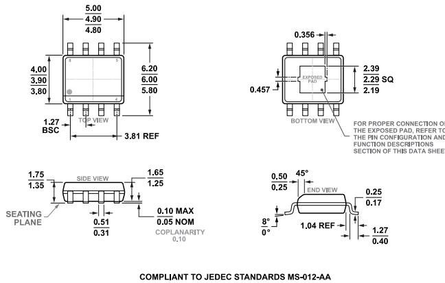
Figure 64. 8-Lead Standard Small Outline Package, with Exposed Pad [SOIC_N_EP] Narrow Body (RD-8-1) Dimensions shown in millimeters
