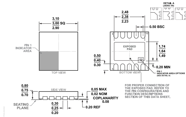
Figure 63. 10-Lead Lead Frame Chip Scale Package [LFCSP] 3 mm x 3 mm Body and 0.75 mm Package Height (CP-10-9) Dimensions shown in millimeters
