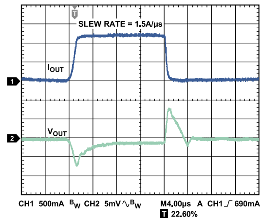
Figure 33. Load Transient Response, I_{LOAD} = 100\text{ mA} to 1.2\text{ A} , V_{OUT} = 3.3\text{ V} , V_{IN} = 4.0\text{ V} , C_{OUT} = 22\text{ }\mu\text{F} , Channel 1 = I_{OUT} , Channel 2 = V_{OUT}
