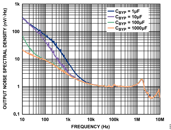
Figure 29. Noise Spectral Density vs. Frequency at Various Values of C_{BYP}
