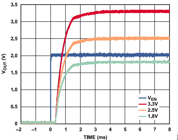
Figure 38. V_{OUT} Start-Up Time After V_{EN} Rising, at Various Output Voltages, V_{IN} = 5\text{ V} , C_{BYP} = 1\text{ }\mu\text{F}
