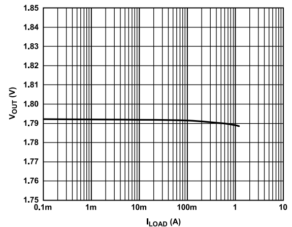
Figure 15. Output Voltage ( V_{OUT} ) vs. Load Current ( I_{LOAD} ), V_{OUT} = 1.8\text{ V}
