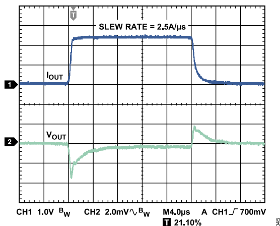
Figure 42. Output Transient Response, V_{OUT} = 3.3\text{ V} , C_{OUT} = 10\ \mu\text{F} , Channel 1 = Load Current, Channel 2 = V_{OUT}
