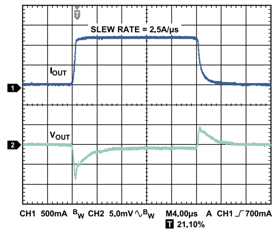
Figure 32. Load Transient Response, I_{LOAD} = 100\text{ mA} to 1.2\text{ A} , V_{OUT} = 3.3\text{ V} , V_{IN} = 4.0\text{ V} , Channel 1 = I_{OUT} , Channel 2 = V_{OUT}
