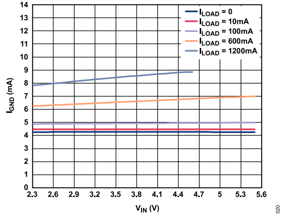
Figure 19. Ground Current ( I_{GND} ) vs. Input Voltage ( V_{IN} ) at Various Loads, V_{OUT} = 1.8\text{ V}
