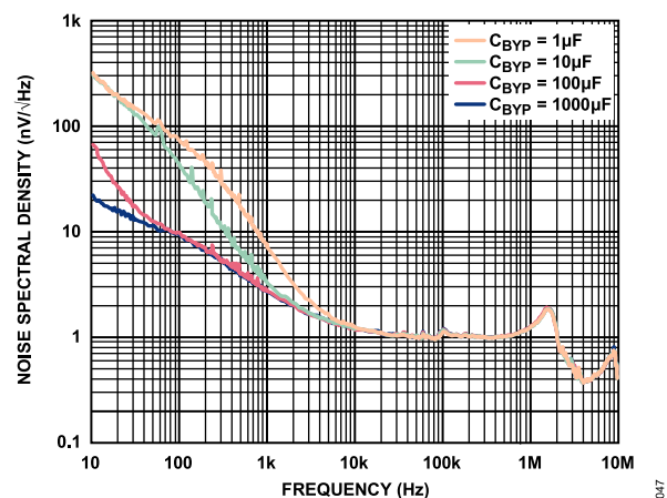
Figure 44. Noise Spectral Density vs. Frequency at Various C_{BYP} Values
