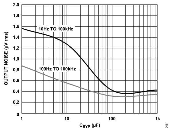
Figure 43. RMS Output Noise vs. Bypass Capacitance ( C_{BYP} )
