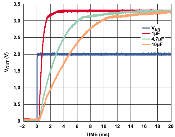
Figure 51. Typical Start-Up Behavior with C_{BYP} = 1\text{ }\mu\text{F} to 10\text{ }\mu\text{F}
