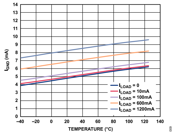
Figure 8. Ground Current ( I_{GND} ) vs. Temperature at Various Loads, V_{OUT} = 3.3\text{ V}
