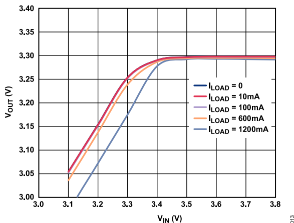
Figure 12. Output Voltage ( V_{OUT} ) vs. Input Voltage ( V_{IN} ) at Various Loads in Dropout, V_{OUT} = 3.3\text{ V}
