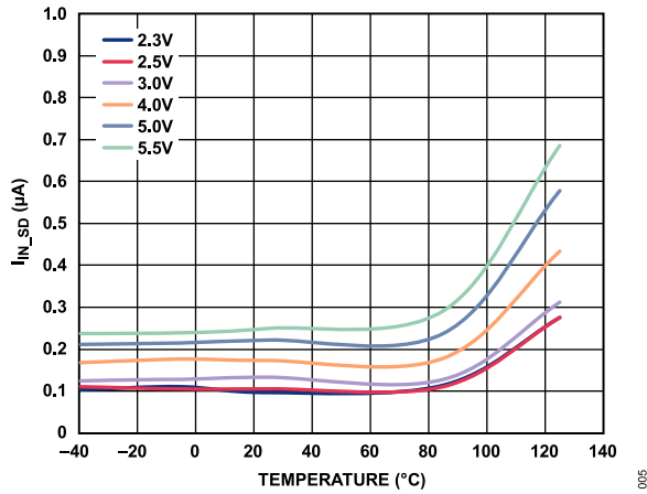
Figure 4. Shutdown Current ( I_{IN\_SD} ) vs. Temperature at Various Input Voltages ( V_{IN} ), V_{OUT} = 1.8\text{ V}
