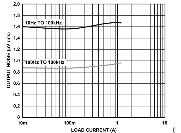
Figure 27. RMS Output Noise vs. Load Current
