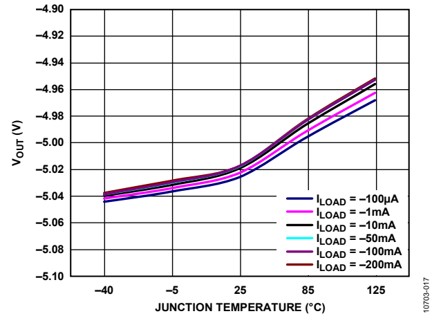
Figure 19. Output Voltage ( V_{OUT} ) vs. Junction Temperature ( T ), V_{OUT} = -5 V
