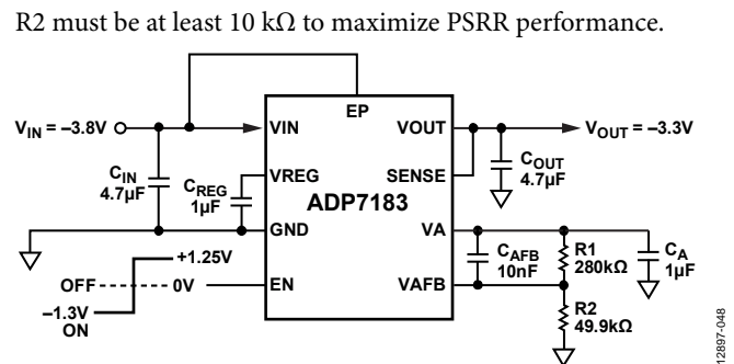
Figure 42. Setting the Adjustable Output Voltage
