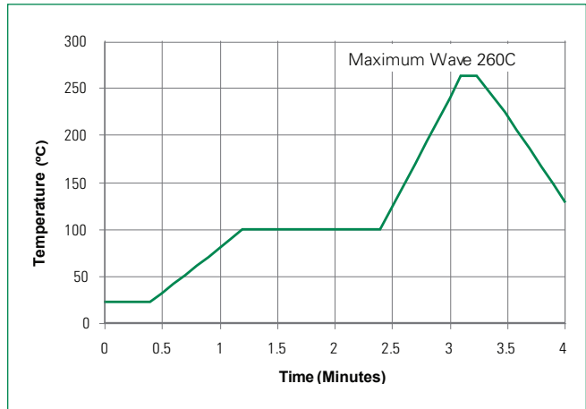
Figure 2- Lead-free Profile
