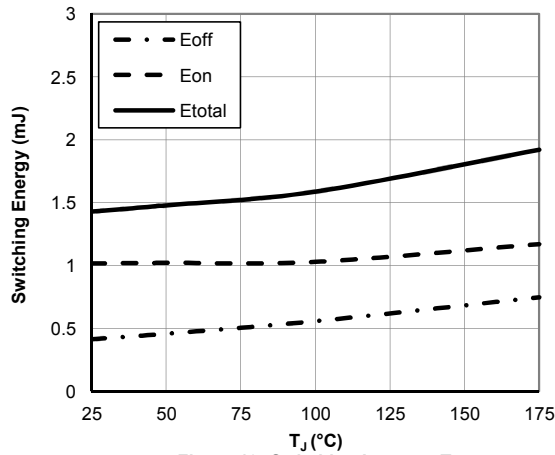
Figure 19: Switching Loss vs. T_J ( V_{GE}=15\text{V} , V_{CE}=400\text{V} , I_C=30\text{A} , R_g=10\Omega )
