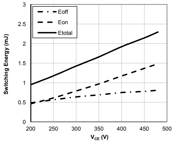
Figure 20: Switching Loss vs. V_{CE} ( T_J=175^\circ\text{C} , V_{GE}=15\text{V} , I_C=30\text{A} , R_g=10\Omega )
