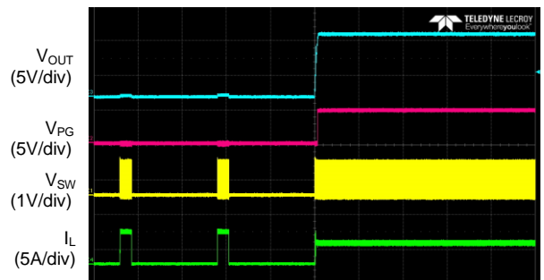
SCP Recovery (I OUT =3A) for AP3441
