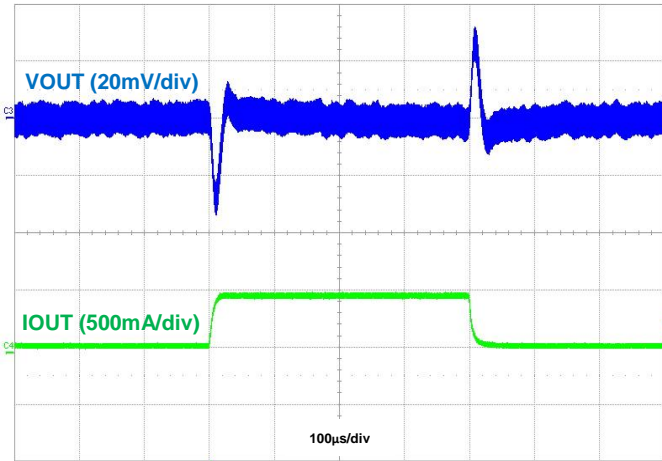
Figure 42. Load Transient, I_{\text{OUT}} = 50\text{mA} to 500\text{mA} to 50\text{mA}
