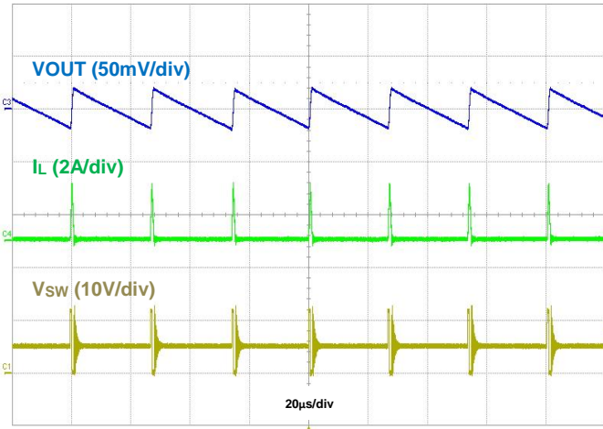
Figure 18. Output Voltage Ripple, I_{OUT} = 50\text{mA}
