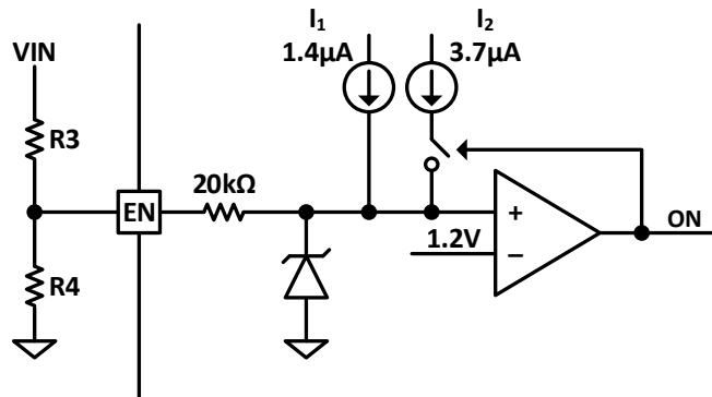
Figure 51. Programming UVLO
