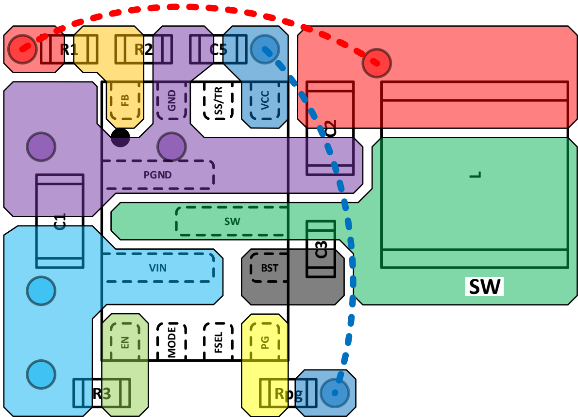
Figure 53. Recommended PCB Layout
