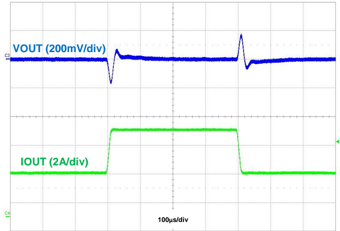
Figure 43. Load Transient, I_{\text{OUT}} = 3\text{A} to 6\text{A} to 3\text{A}
