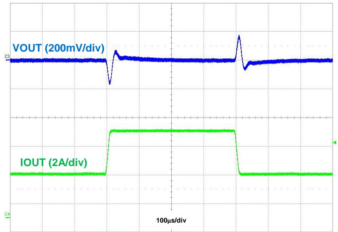
Figure 21. Load Transient, I_{OUT} = 3\text{A} to 6\text{A} to 3\text{A}
