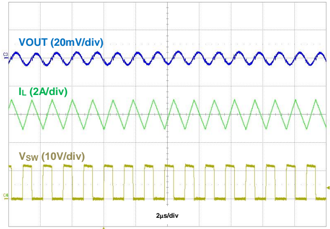
Figure 30. Output Voltage Ripple, I_{OUT} = 6\text{A}
