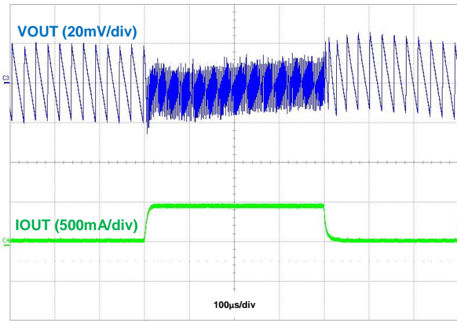
Figure 31. Load Transient, I_{OUT} = 50\text{mA} to 500\text{mA} to 50\text{mA}
