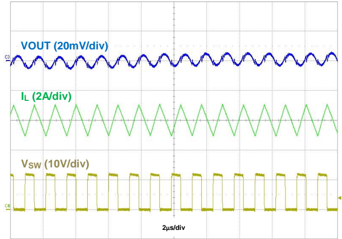
Figure 41. Output Voltage Ripple, I_{\text{OUT}} = 6\text{A}
