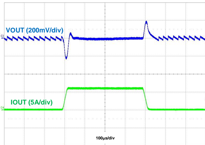
Figure 22. Load Transient, I_{OUT} = 50\text{mA} to 6\text{A} to 50\text{mA}
