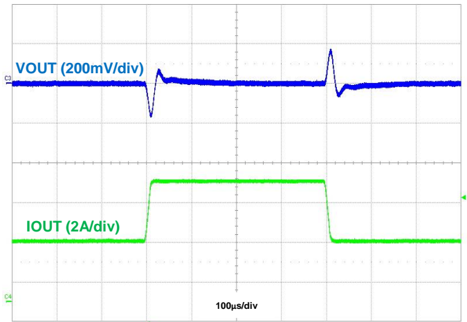
Figure 32. Load Transient, I_{OUT} = 3\text{A} to 6\text{A} to 3\text{A}
