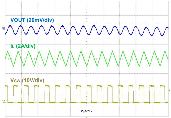
Figure 19. Output Voltage Ripple, I_{OUT} = 6\text{A}
