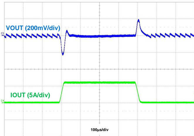
Figure 33. Load Transient, I_{OUT} = 50\text{mA} to 6\text{A} to 50\text{mA}
