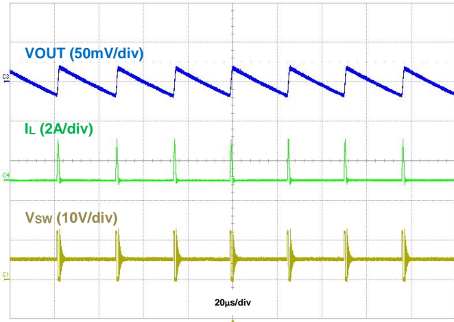
Figure 29. Output Voltage Ripple, I_{OUT} = 50\text{mA}
