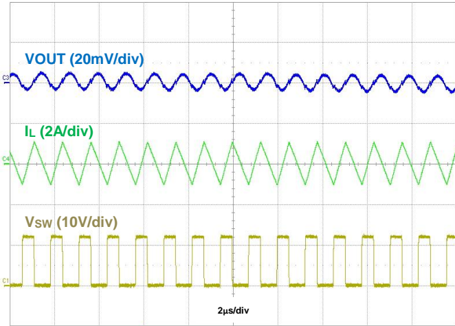
Figure 40. Output Voltage Ripple, I_{\text{OUT}} = 50\text{mA}
