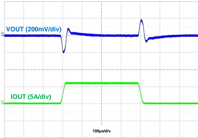
Figure 44. Load Transient, I_{\text{OUT}} = 50\text{mA} to 6\text{A} to 50\text{mA}
