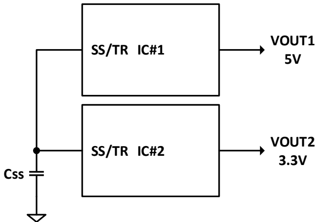
Figure 45. Ratiometric Tracking Configuration
