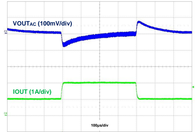
Figure 52. Load Transient, I_{OUT} = 1\text{A} to 2A to 1A
