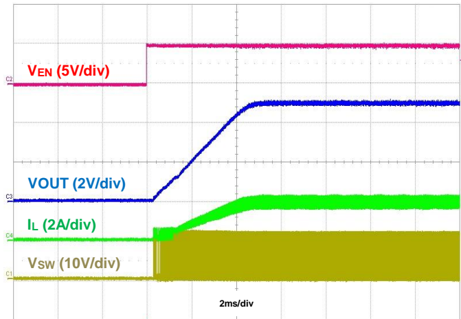
Figure 11. Startup using EN, IOUT = 2A
