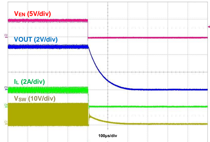
Figure 12. Shutdown using EN, IOUT = 2A
