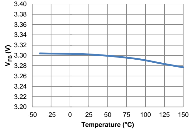
Figure 46. Feedback Voltage vs. Temperature, IOUT = 1A
