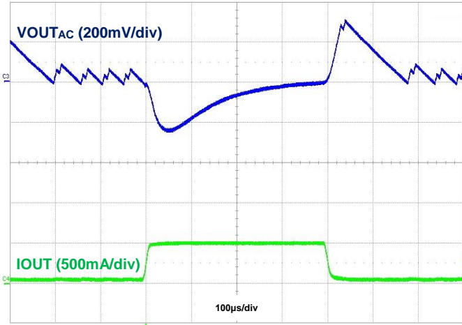
Figure 26. Load Transient, IOUT = 50mA to 500mA to 50mA
