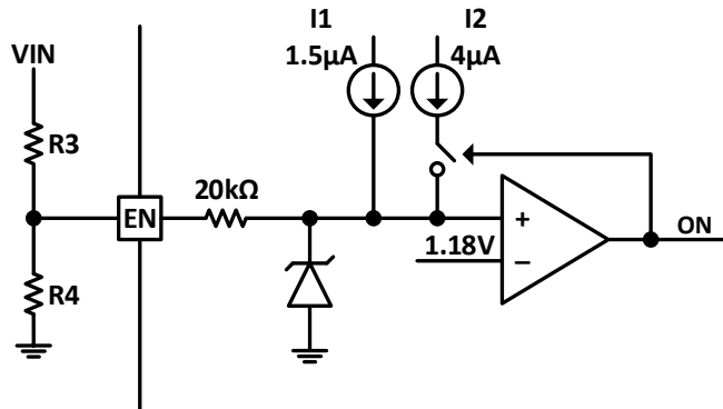
Figure 74. Adjusting UVLO
