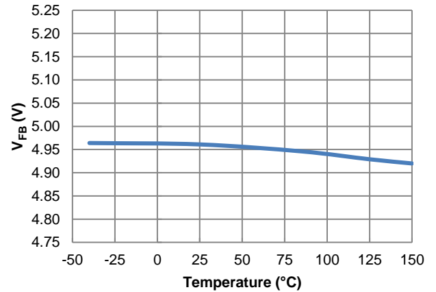
Figure 61. Feedback Voltage vs. Temperature, IOUT = 1A
