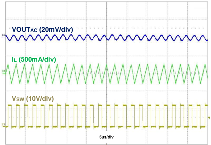
Figure 36. Output Voltage Ripple, V_{OUT} = 5\text{V} , I_{OUT} = 50\text{mA}
