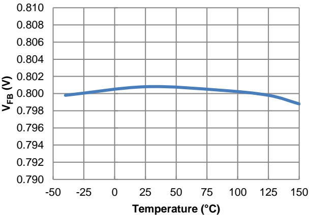
Figure 15. Feedback Voltage vs. Temperature, IOUT = 1A
