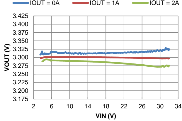
Figure 44. Line Regulation
