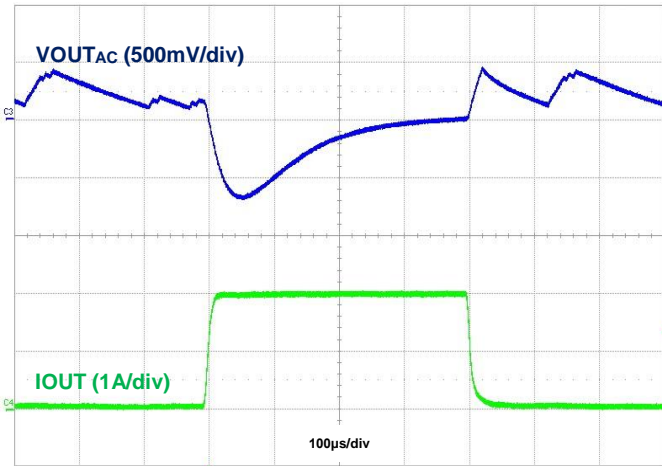
Figure 28. Load Transient, IOUT = 50mA to 2A to 50mA
