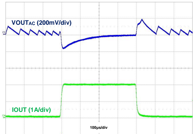
Figure 53. Load Transient, I_{OUT} = 50\text{mA} to 2A to 50mA
