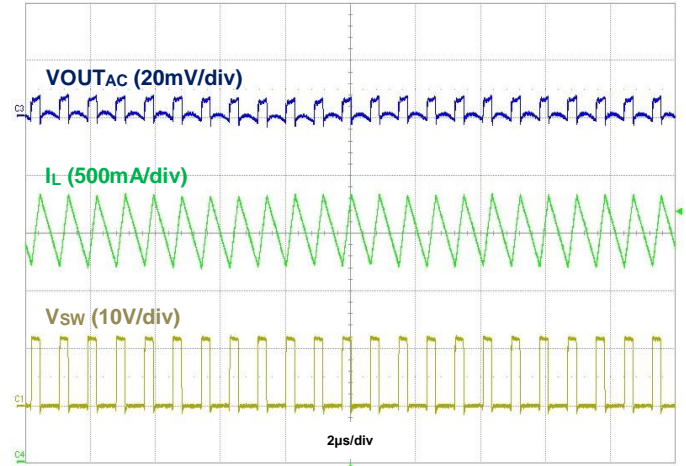
Figure 50. Output Voltage Ripple, I_{OUT} = 2\text{A}
