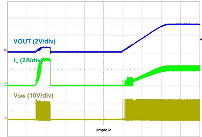
Figure 57. Output Short Recovery, IOU = 2A
