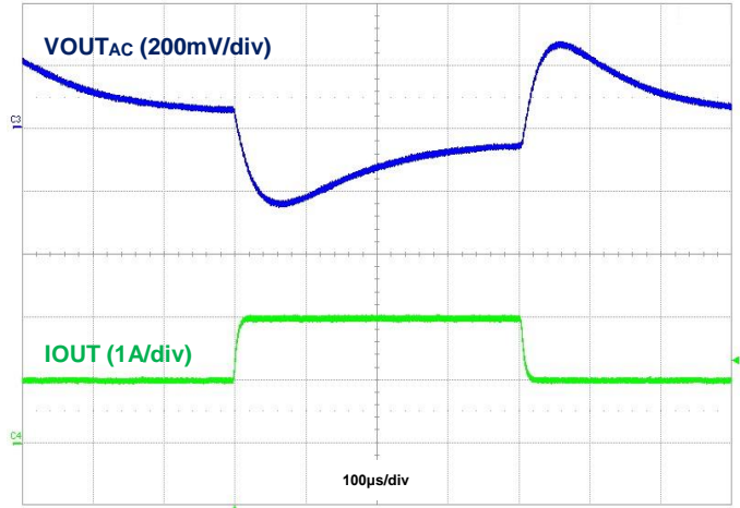
Figure 27. Load Transient, IOUT = 1A to 2A to 1A
