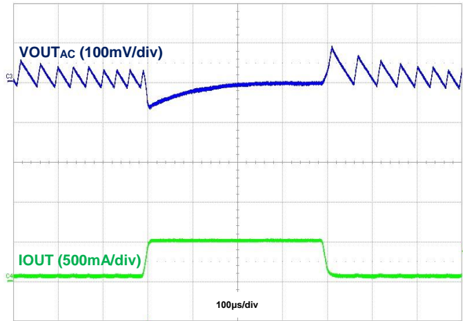
Figure 51. Load Transient, I_{OUT} = 50\text{mA} to 500mA to 50mA
