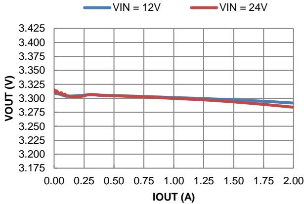
Figure 45. Load Regulation
