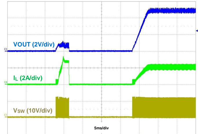
Figure 14. Output Short Recovery, IOUT = 2A
