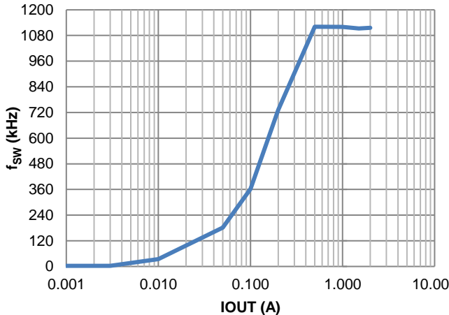
Figure 48. f_{sw} vs. Load
