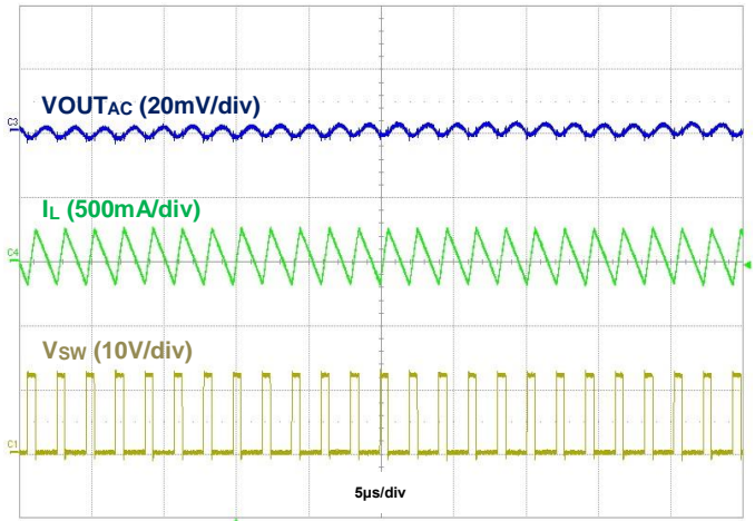
Figure 38. Output Voltage Ripple, V_{OUT} = 3.3\text{V} , I_{OUT} = 50\text{mA}
