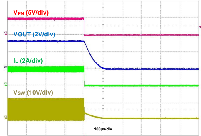
Figure 55. Shutdown using EN, IOU = 2A
