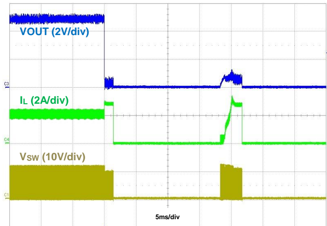
Figure 13. Output Short Protection, IOUT = 2A
