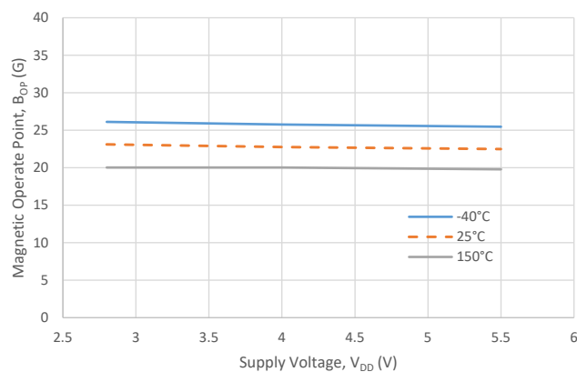
Operate Point (B) vs. Supply Voltage
