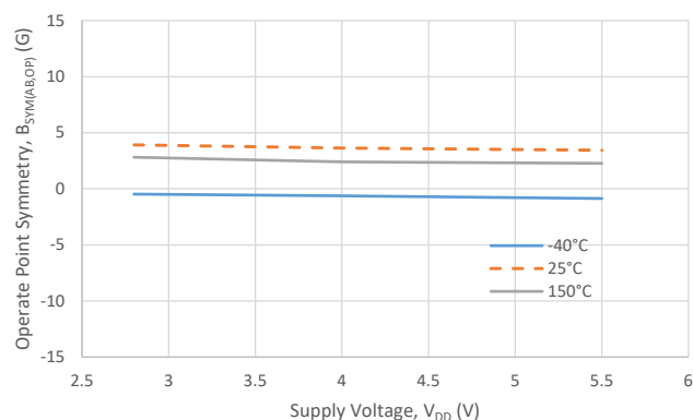
Operate Symmetry (AB) vs. Supply Voltage
