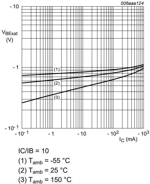
Fig. 13. BC807-40W: Base-emitter saturation voltage as a function of collector current; typical values
